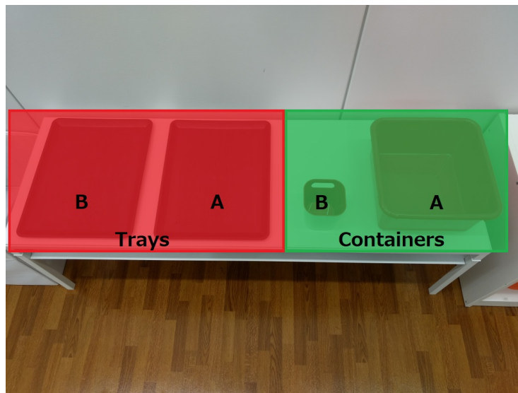
Figure 19: In the Deposit Area, on the Long Table A there will be four deposits: Tray A, Tray B, Container A, and Container B. As a reference, the tray's size is 0.38 x 0.36 m, Container A is 0.28 x 0.28 x 0.125 m, and Container B is 0.095 x 0.095 m and 0.105 m height. Single color deposits are considered to detect any tag or mark that might be used as a reference.
